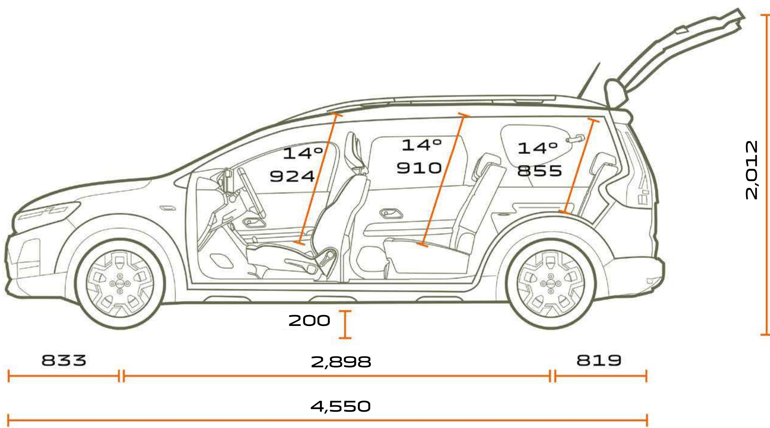
SIDE VIEW 7-SEATER
