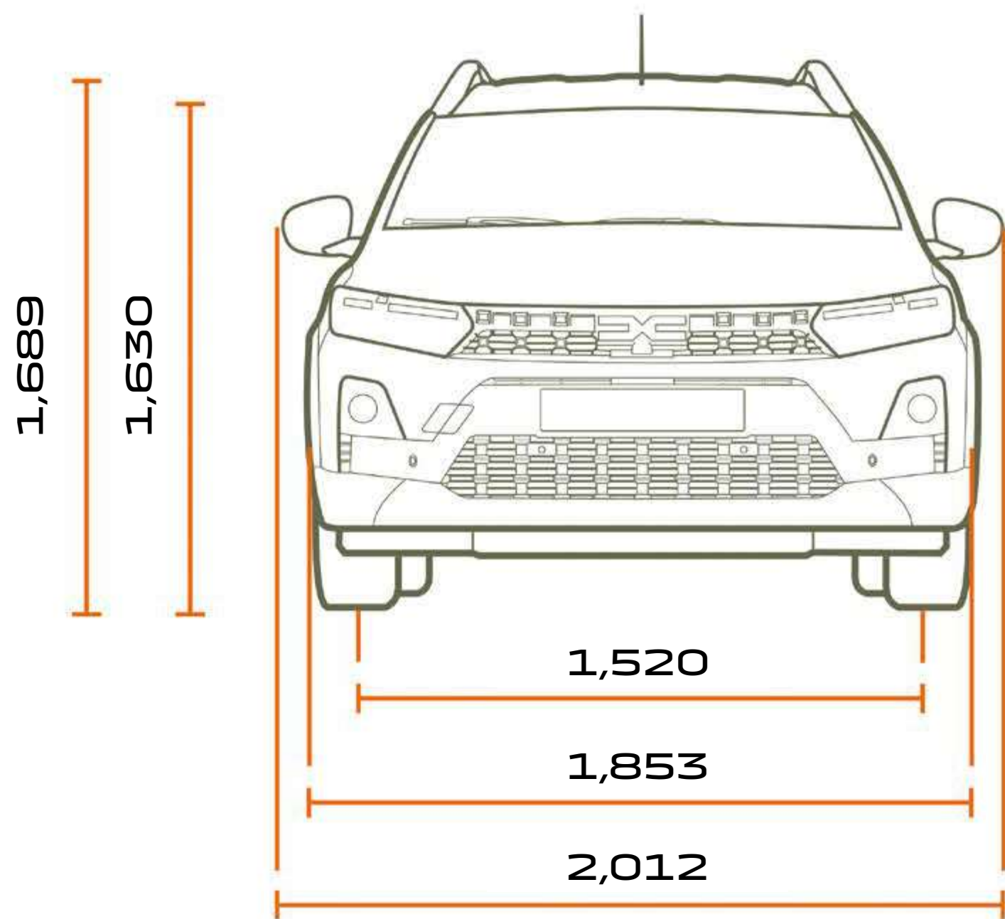
FRONT VIEW 7-SEATER
